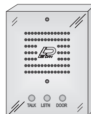
IR-443SS Surface Mount Version With Round Buttons
