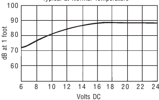
DECIBELS VS. VOLTAGE FOR LUMATONE AUDIO SIGNALS Typical at Normal Temperature
