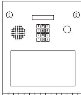
1810 Flush 12" W x 13.25" H x 3" D 30.4cm W x 33.65cm H x 7.62cm D
